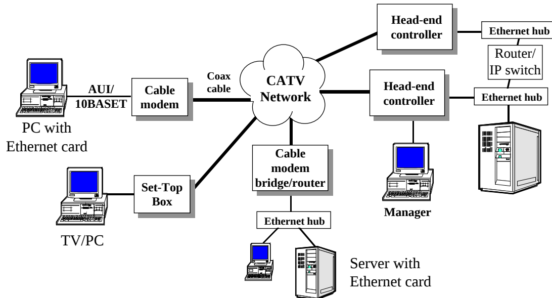
Figure 1 A cable modem architecture.
