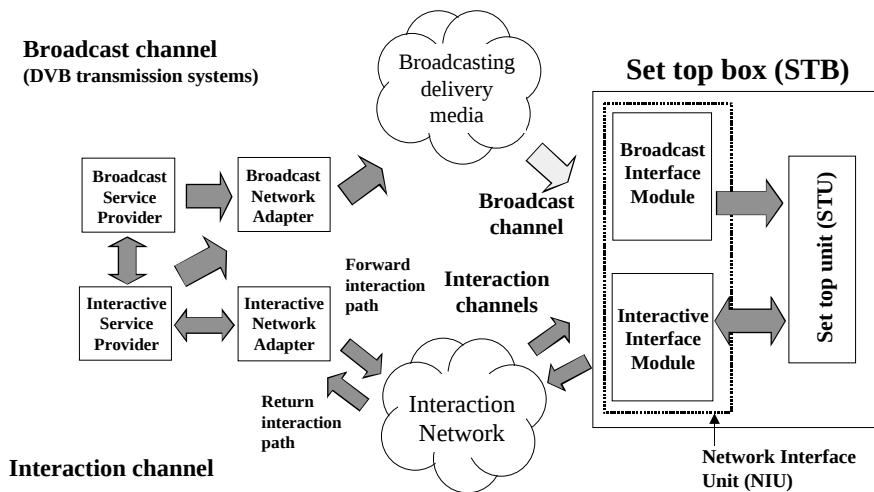
Figure 3 The DVB/DAVIC reference model.
