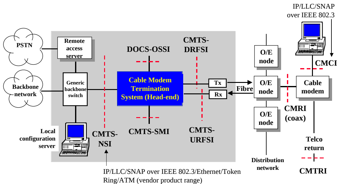
Figure 2 The DOCSIS reference model.
